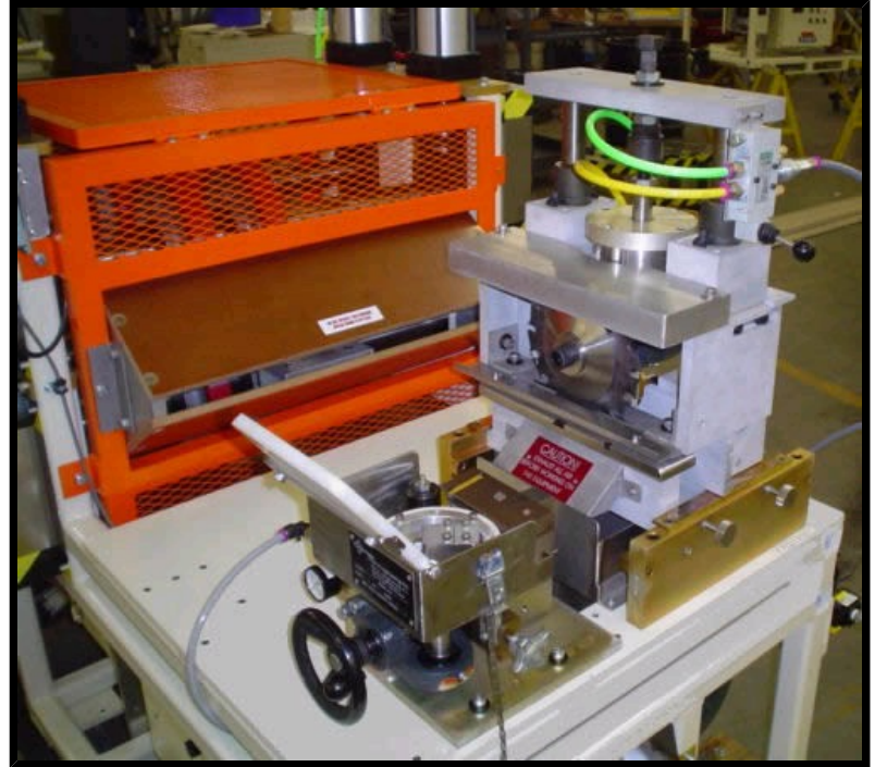
Puller with Nail & Weep Hole Punches
